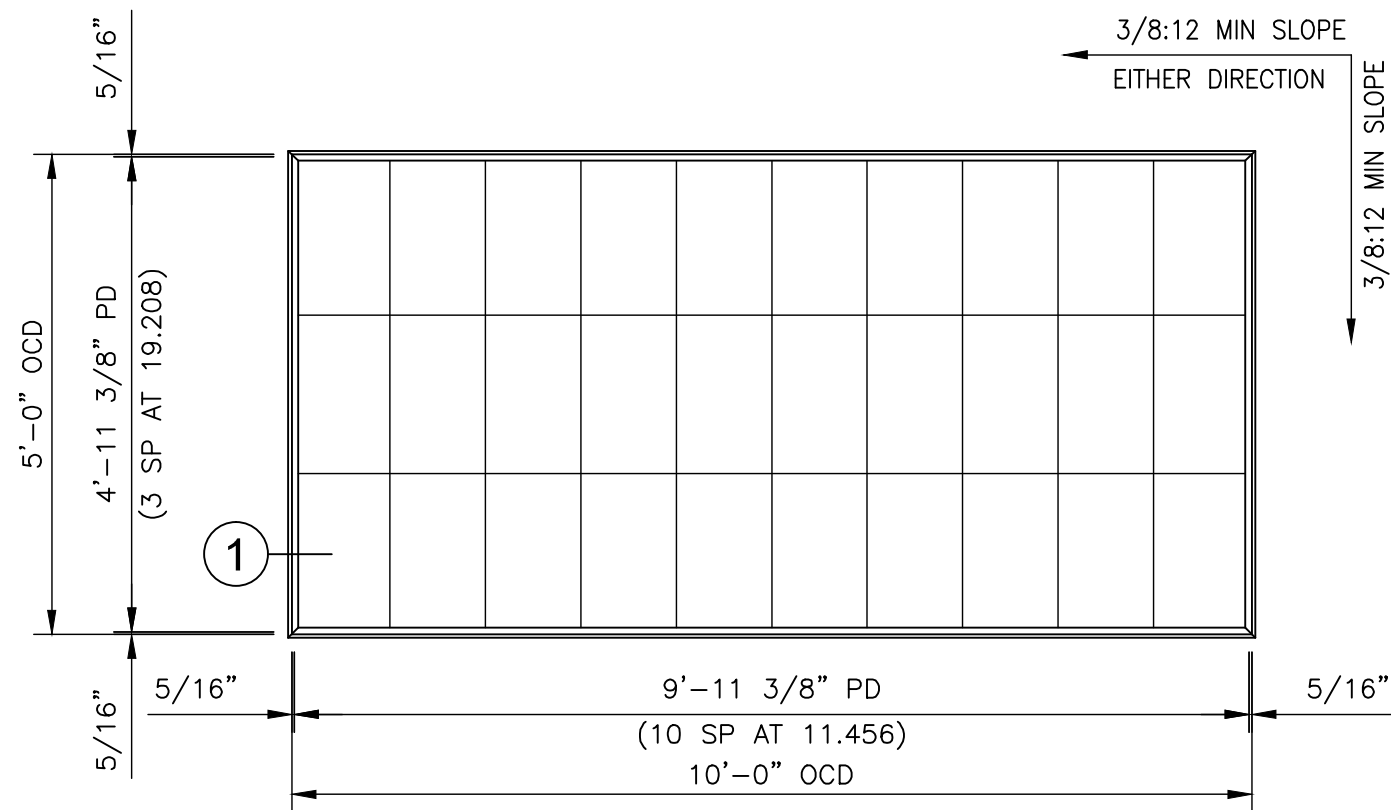
5' x 10' SKYLIGHT S-510-3A
