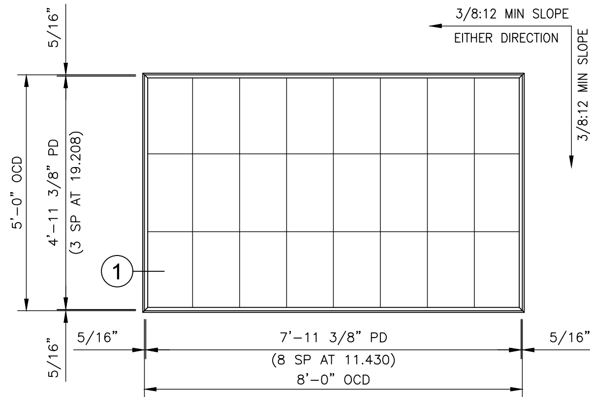
5' x 8' SKYLIGHT S-58-3A
