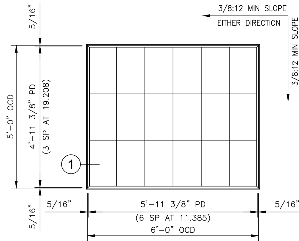
5' x 6' SKYLIGHT S-56-3A
