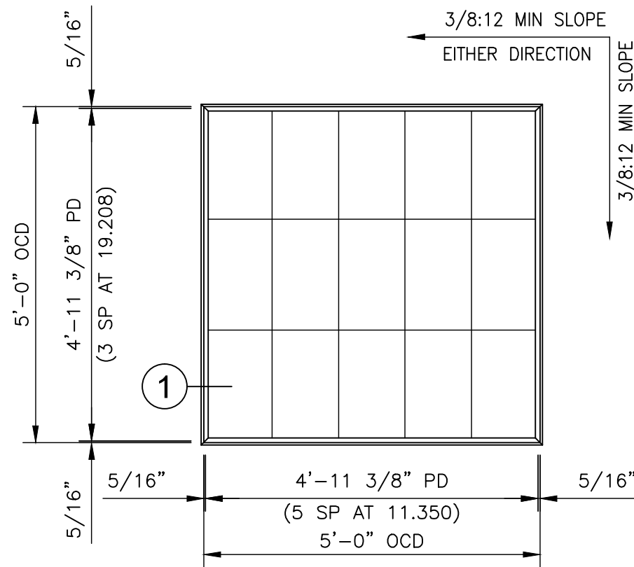
5' x 5' SKYLIGHT S-55-3A
