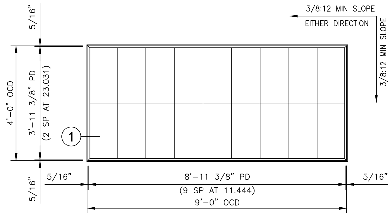
4' x 9' SKYLIGHT S-49-3A
