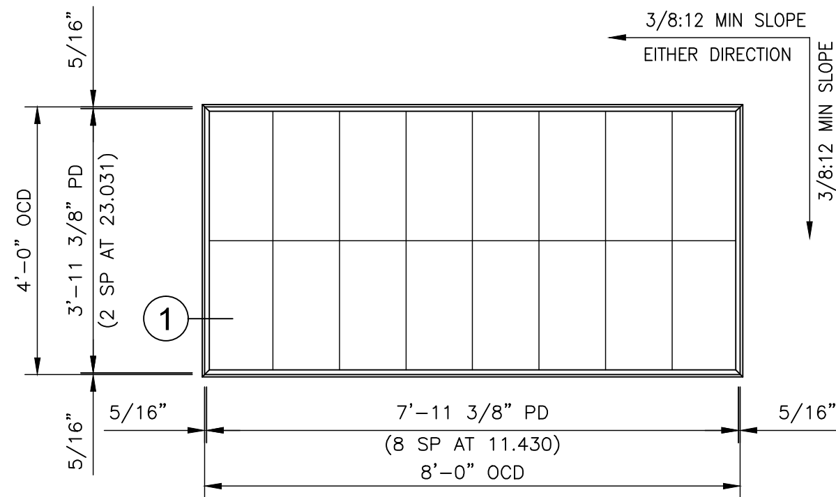
4' x 8' SKYLIGHT S-48-3A
