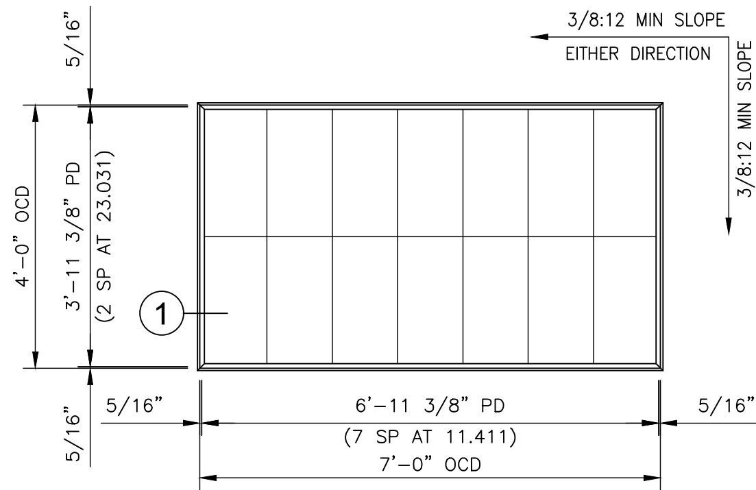
4' x 7' SKYLIGHT S-47-3A
