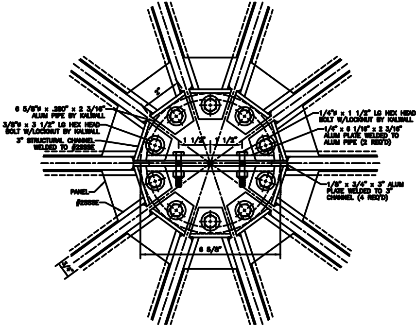
AA COMPRESSION RING PLAN VIEW
