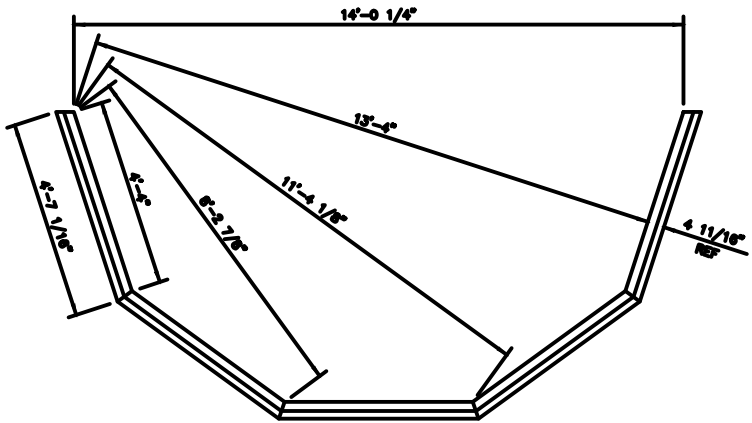
INSTALLATION DIMENSIONS FOR CURB CAP LAYOUT OF HALF THE GEO ROOF
