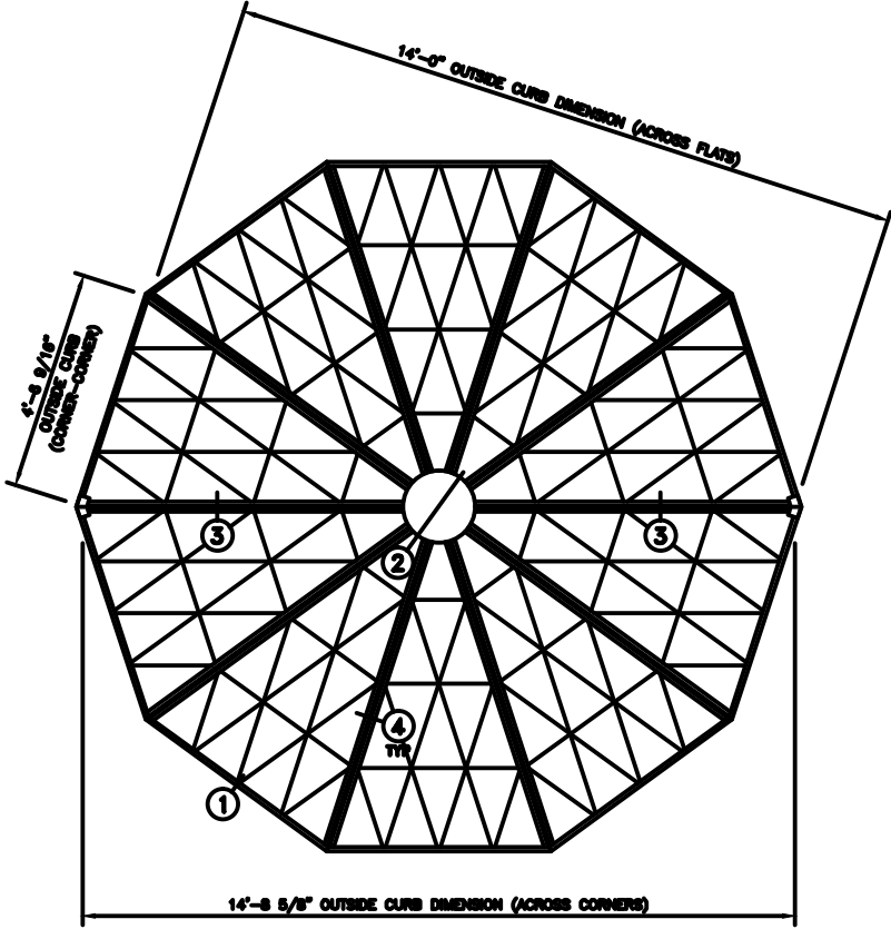
GEO ROOF PLAN NOTE: SHIPPED IN 2 UNITS
